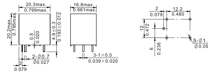
Mounting (Bottom view)
